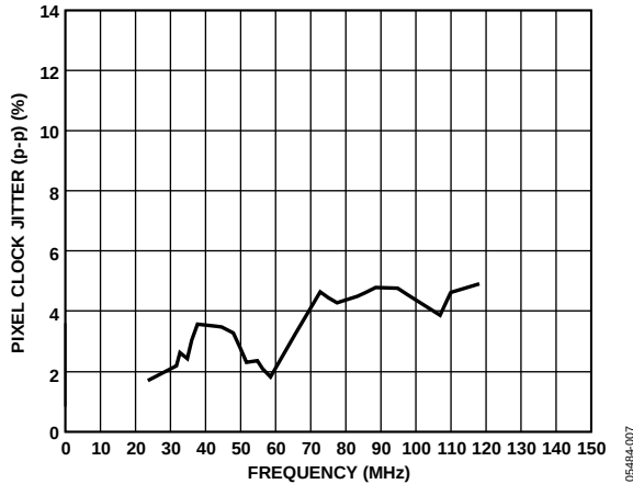
Figure 7. Pixel Clock Jitter vs. Frequency
