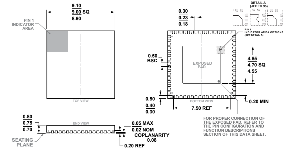
Figure 21. 64-Lead Lead Frame Chip Scale Package [LFCSP] 9 mm × 9 mm Body and 0.75 mm Package Height (CP-64-21)
