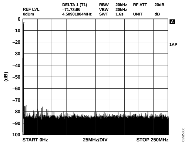
Figure 4. Wideband SFDR, f_{OUT} = 1.1 MHz, f_{CLK} = 500 MSPS
