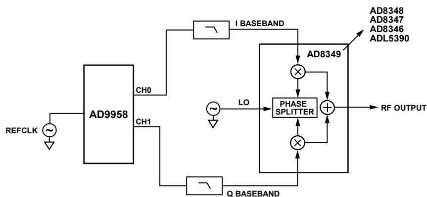
Figure 23. Single-Sideband-Suppressed Carrier Upconversion
