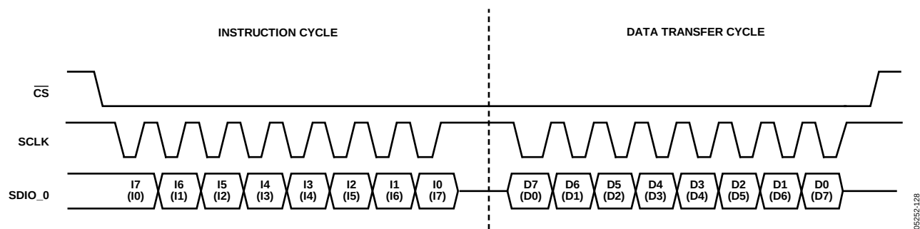
Figure 46. Single-Bit Serial Mode (2-Wire) Read Timing—Clock Stall High
