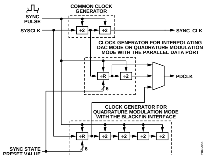
Figure 55. Clock Generator
