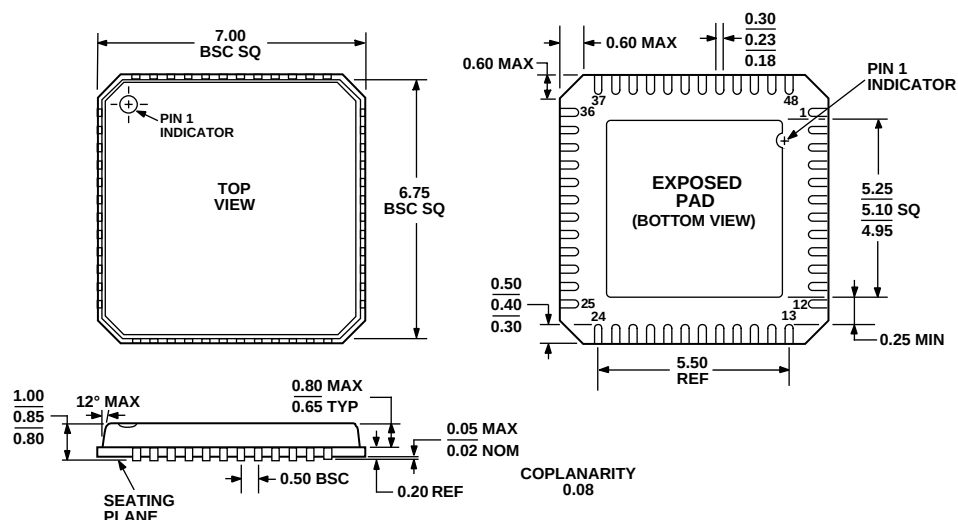
Figure 35. 48-Lead Lead Frame Chip Scale Package [LFCSP] 7 mm x 7 mm Body (CP-48) Dimensions shown in millimeters
