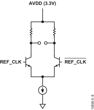
Figure 27. REF CLK input
