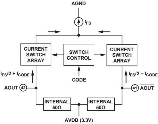
Figure 26. DAC Output
