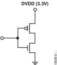
Figure 28. CMOS Input
