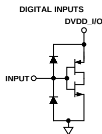
Figure 3. Equivalent Input Circuit
