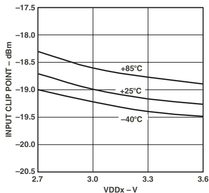
TPC 4b. Maximum VGA Attenuation Clip Point vs. Supply (High Bias 2 )
