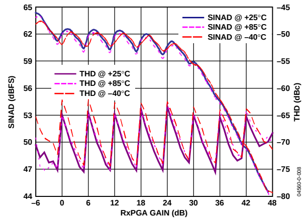
Figure 8. SINAD/THD Performance vs. R_{\text{xPGA}} Gain and Temperature ( f_{\text{IN}} = 5 MHz)
