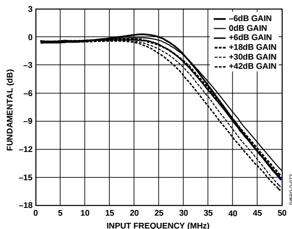
Figure 72. Effects of RxPGA Gain on LPF Frequency Response ( f_{-3\text{ dB}} = 32\text{ MHz} (@ 0\text{ dB} and f_{\text{ADC}} = 80\text{ MSPS} )
