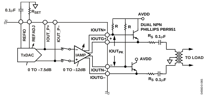
Figure 65. Voltage-Mode Operation
