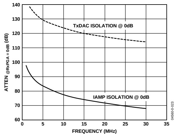
Figure 23. Rx to Tx Full-Duplex Isolation @ 0 RxPGA Setting (Note: \text{ATTEN}_{\text{@RxPGA} = x\text{ dB}} = \text{ATTEN}_{\text{@RxPGA} = 0\text{ dB}} - \text{RxPGA Gain} )
