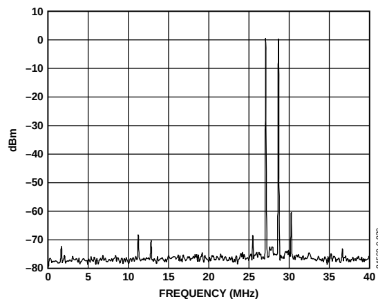
Figure 30. Dual-Tone Spectral Plot of TxDAC's Output ( f_{\text{DATA}} = 80 MSPS, 2 \times Interpolation, 10 dBm Peak Power, F_1 = 27.1 MHz, F_2 = 28.7 MHz)
