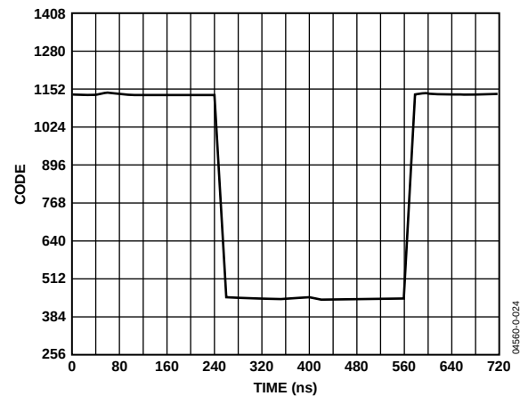
Figure 24. RxPGA Settling Time for 0 dB to +5 dB Transition for DC Input ( f_{\text{ADC}} = 50 MSPS, LPF Disabled)
