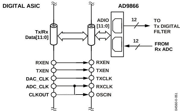
Figure 51. Example of a Half-Duplex Digital Interface with AD9866 Serving as the Slave
