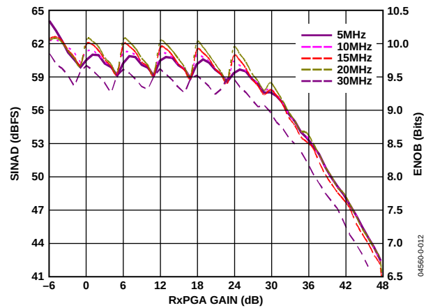
Figure 12. SINAD/ENOB vs. R_{\text{xPGA}} Gain and Frequency
