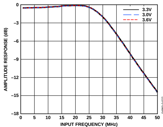
Figure 22. Rx Low-Pass Filter Amplitude Response vs. Supply ( f_{\text{ADC}} = 50 MSPS, f_{-3\text{ dB}} = 33 MHz, RxPGA = 0 dB)
