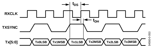
Figure 53. Tx[5:0] Port Full-Duplex Timing Diagram
