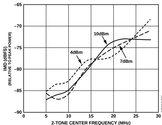
Figure 31. 2-Tone IMD Frequency Sweep vs. Peak Power with f_{\text{DATA}} = 80 MSPS, 2 \times Interpolation
