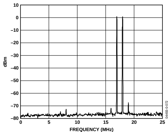
Figure 27. Dual-Tone Spectral Plot of TxDAC's Output ( f_{\text{DATA}} = 50 MSPS, 4 \times Interpolation, 10 dBm Peak Power, F_1 = 17 MHz, F_2 = 18 MHz)
