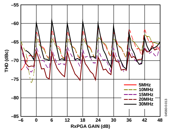
Figure 13. THD vs. R_{\text{xPGA}} Gain and Frequency
