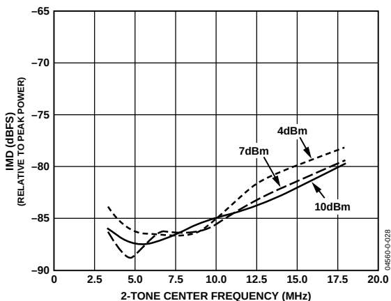
Figure 28. 2-Tone IMD Frequency Sweep vs. Peak Power with f_{\text{DATA}} = 50 MSPS, 4 \times Interpolation
