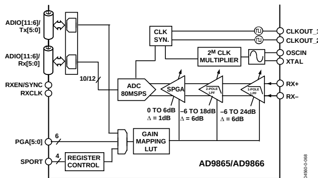
Figure 68. Functional Block Diagram of Rx Path
