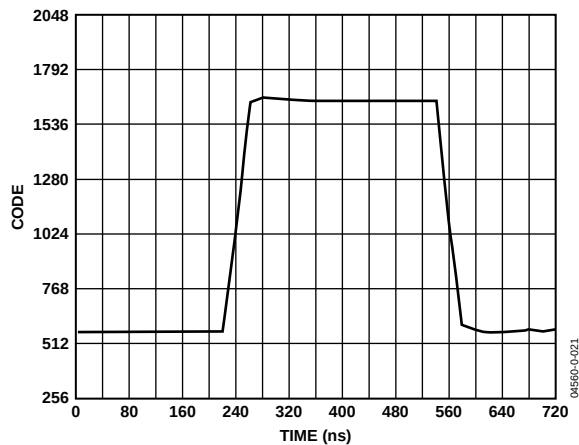
Figure 21. RxPGA Settling Time -12 dB to +48 dB Transition for DC Input ( f_{\text{ADC}} = 50 MSPS, LPF Disabled)
