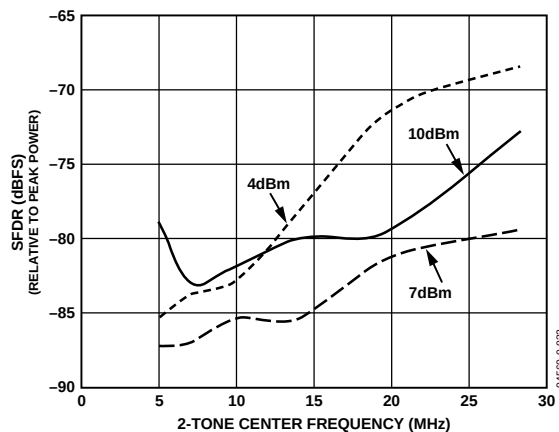
Figure 32. 2-Tone Worst Spur Frequency Sweep vs. Peak Power with f_{\text{DATA}} = 80 MSPS, 2 \times Interpolation
