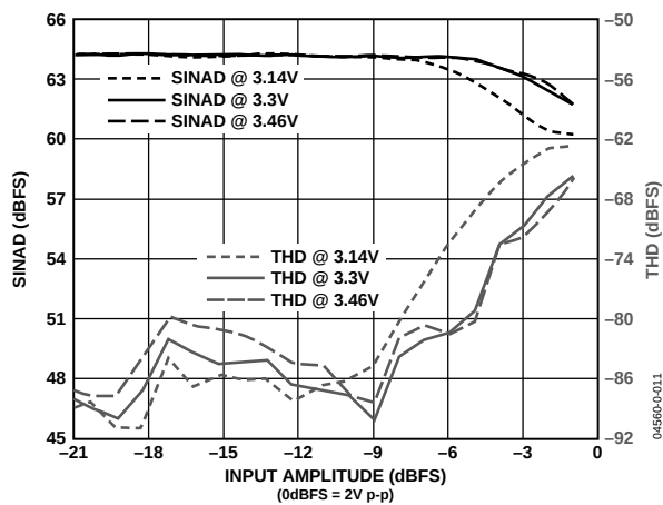
Figure 11. SINAD and THD vs. Input Amplitude and Supply ( f_{\text{IN}} = 8 MHz, LPF f_{-3\text{dB}} = 26 MHz; R_{\text{xPGA}} = 0 dB)
