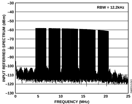
Figure 4. Spectral Plot with 4k FFT of 84-Carrier DMT Signal with \text{PAR} = 10.2 dB, P_{\text{IN}} = -33.7 dBm, and R_{\text{xPGA}} = 36 dB
