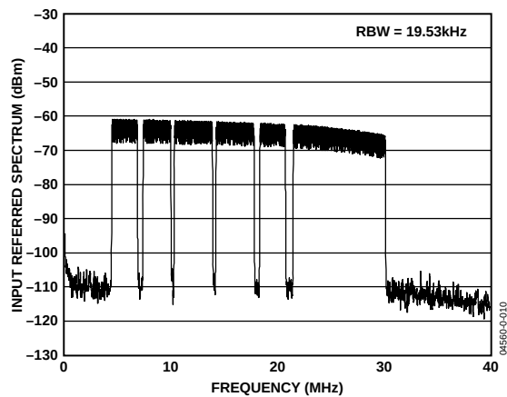
Figure 10. Spectral Plot with 4K FFT of 111-Carrier DMT Signal with \text{PAR} = 11 dB, P_{\text{IN}} = -33.7 dBm, LPF's f_{-3\text{dB}} = 32 MHz and R_{\text{xPGA}} = 36 dB
