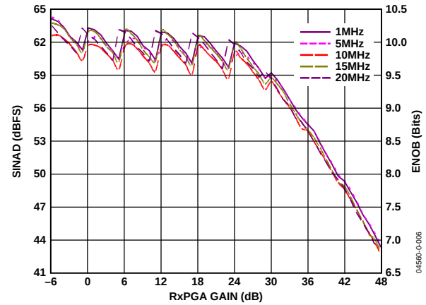
Figure 6. SINAD/ENOB vs. R_{\text{xPGA}} Gain and Frequency
