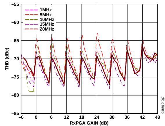
Figure 7. THD vs. R_{\text{xPGA}} Gain and Frequency
