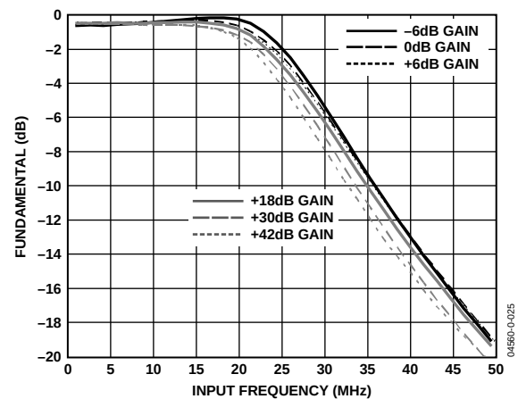
Figure 25. Rx Low-Pass Filter Amplitude Response vs. RxPGA Gain (LPF's f_{-3\text{ dB}} = 33 MHz)
