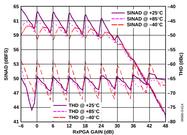
Figure 14. SINAD/THD Performance vs. R_{\text{xPGA}} Gain and Temperature ( f_{\text{IN}} = 10 MHz)
