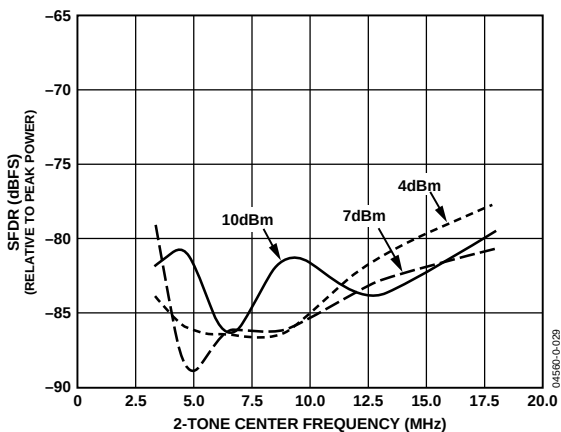
Figure 29. 2-Tone Worst Spur Frequency Sweep vs. Peak Power with f_{\text{DATA}} = 50 MSPS, 4 \times Interpolation
