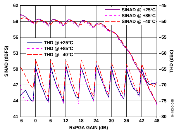
Figure 8. SINAD/THD Performance vs. R_{\text{PGA}} Gain and Temperature ( f_{\text{IN}} = 5 MHz)
