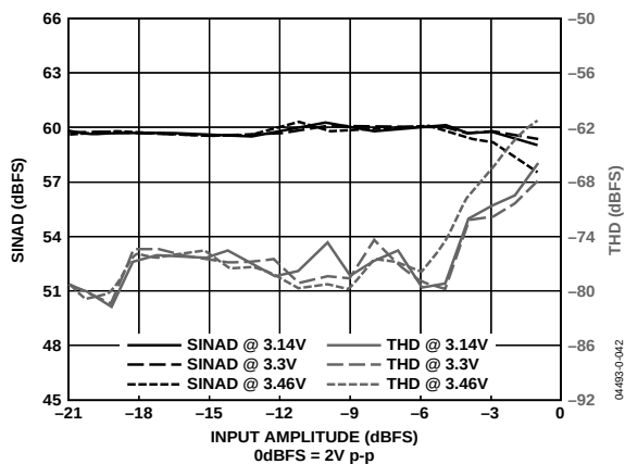
Figure 5. SINAD and THD vs. Input Amplitude and Supply ( f_{\text{IN}} = 8 MHz, LPF f_{-3\text{dB}} = 26 MHz; R_{\text{PGA}} = 0 dB)
