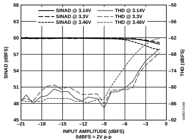
Figure 11. SINAD and THD vs. Input Amplitude and Supply ( f_{\text{IN}} = 8 MHz, LPF f_{-3\text{dB}} = 26 MHz; RxPGA = 0 dB)
