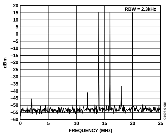
Figure 39. Dual-Tone Spectral Plot of IAMPN Output (IAMP Settings of I = 12.5 mA, N = 4 , G = 0 , 2:1 Transformer into 75 \Omega Loader, V_{\text{CM}} = 4.8 V)
