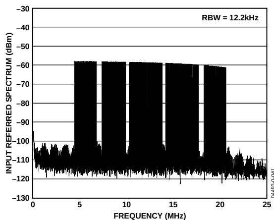
Figure 4. Spectral Plot with 4 k FFT of 84-Carrier DMT Signal with \text{PAR} = 10.2 dB, P_{\text{IN}} = -33.7 dBm, and R_{\text{PGA}} = 36 dB
