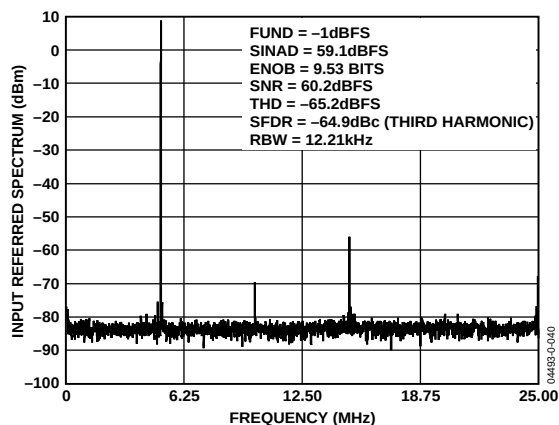
Figure 3. Spectral Plot with 4 k FFT of Input Sinusoid with R_{\text{PGA}} = 0 dB and P_{\text{IN}} = 9 dBm
