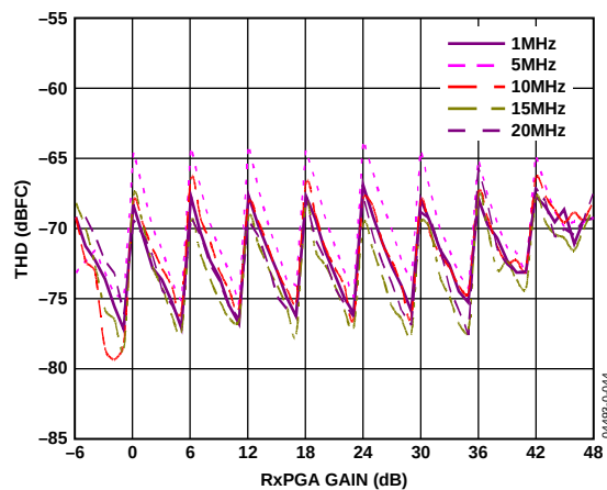
Figure 7. THD vs. R_{\text{PGA}} Gain and Frequency
