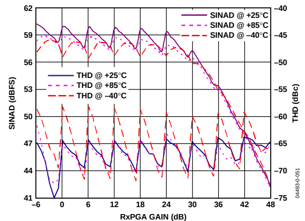
Figure 14. SINAD/THD Performance vs. RxPGA Gain and Temperature ( f_{\text{IN}} = 10 MHz)
