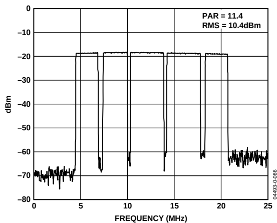
Figure 41. Spectral Plot of 84-Carrier OFDM Test Vector Using IAMP in Voltage-Mode Configuration with AV_{\text{DD}} = 5 V (PBR951 Transistors, IAMP Settings of I = 6 mA, N = 2 , G = 6 )
