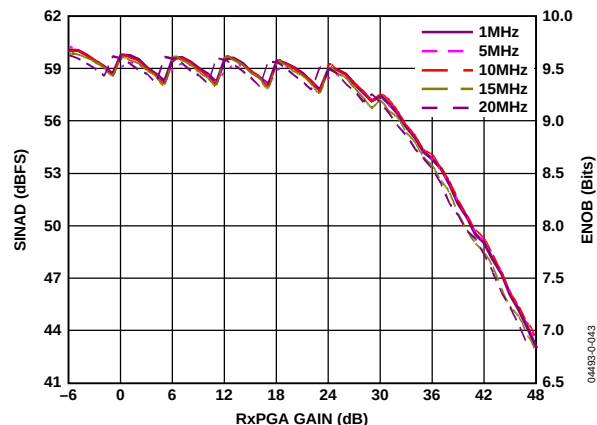
Figure 6. SINAD/ENOB vs. R_{\text{PGA}} Gain and Frequency
