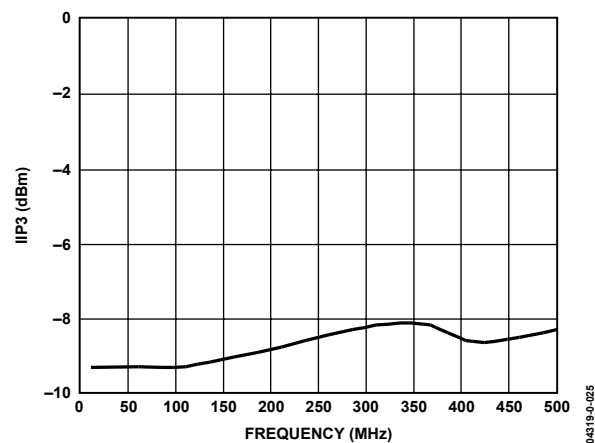
Figure 25. Input IIP3 vs. Frequency ( f_{CLK} = 18\text{ MSPS} )
