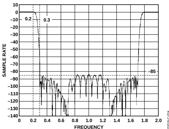
Figure 24. Half-Band 1 and 2 Frequency Response; Frequency Relative to HB1 Output Sample Rate
