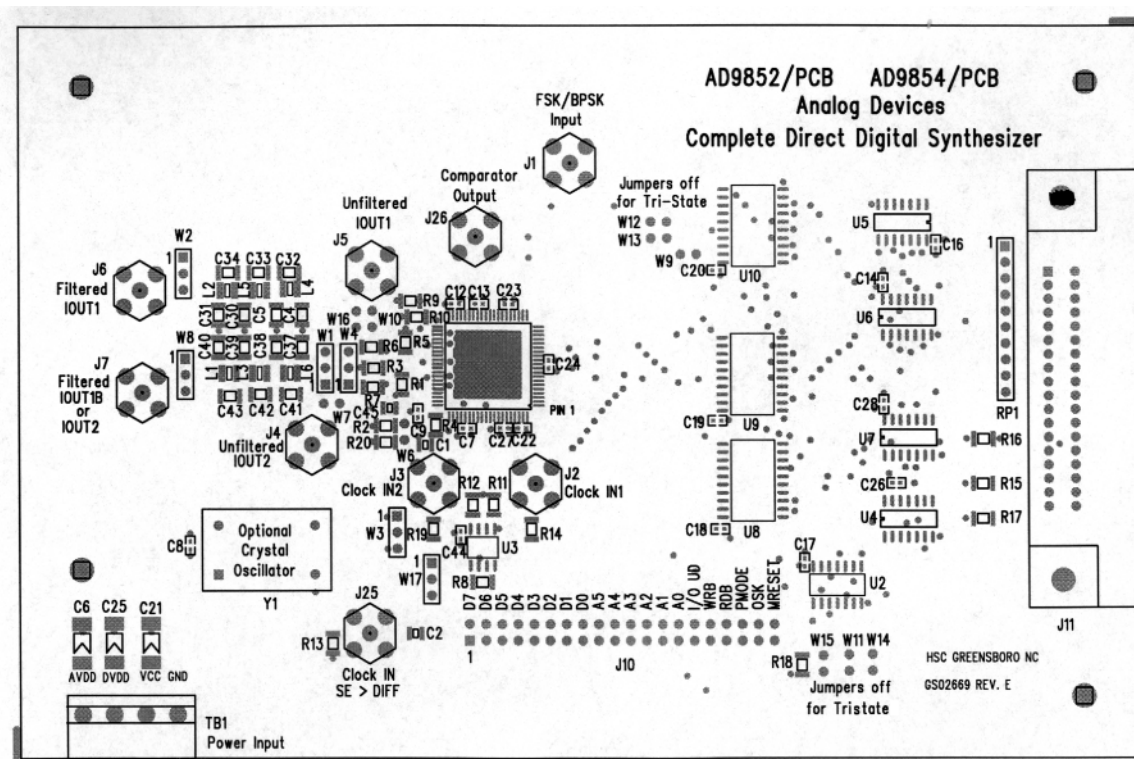
Figure 63. Assembly Drawing
