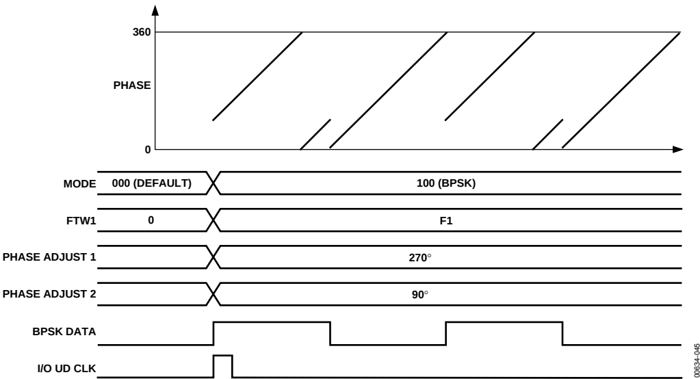
Figure 45. BPSK Mode
