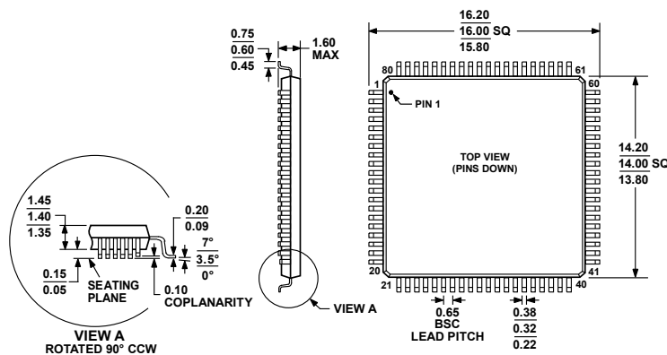
Figure 61. 80-Lead Thin Quad Flat Package, Exposed Pad [TQFP_EP] (SV-80-4) Dimensions shown in millimeters
