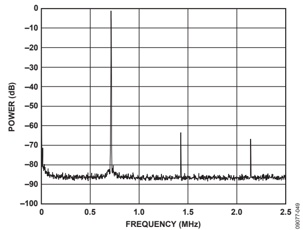
Figure 17. Power vs. Frequency, f_{CLK} = 5 MHz, f_{OUT} = 0.714 MHz = f_{CLK}/7 , Frequency Word = 0x2492492
