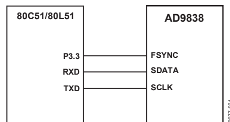
Figure 29. 80C51/80L51 to AD9838 Interface
