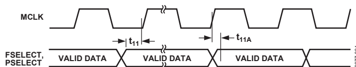
Figure 3. Control Timing
