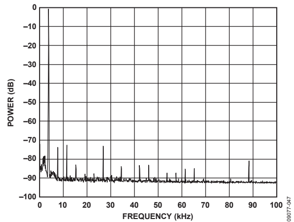
Figure 15. Power vs. Frequency, f_{CLK} = 16 MHz, f_{OUT} = 3.8 kHz, Frequency Word = 0x000FBA9
