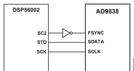
Figure 30. DSP56002 to AD9838 Interface
