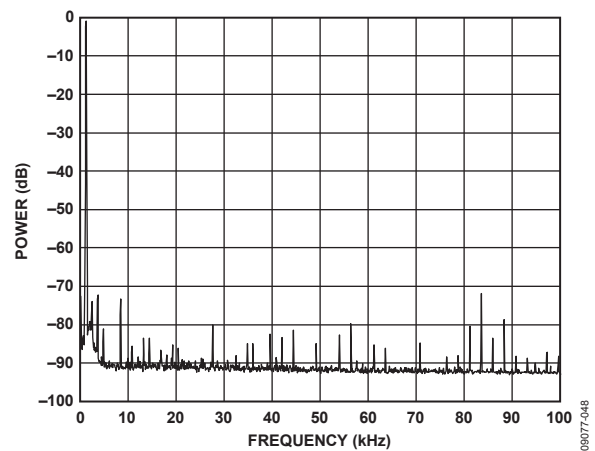
Figure 16. Power vs. Frequency, f_{CLK} = 5 MHz, f_{OUT} = 1.2 kHz, Frequency Word = 0x000FBA9
