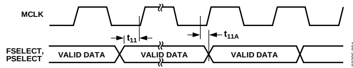
Figure 4. Control Timing
