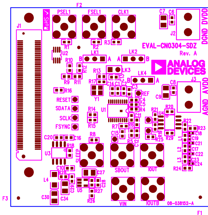
EVAL-CN-304-SDZ (08-038152-A) – Component Side View Silkscreen
