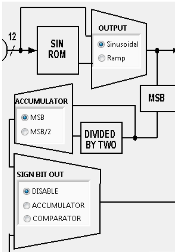
Figure 9. Waveform Profile and SIGN BIT OUT
