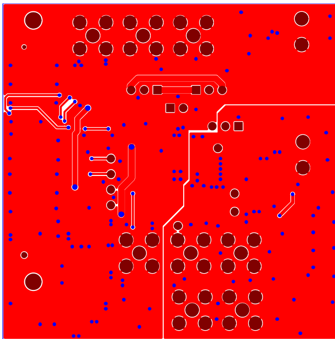
EVAL-CN-304-SDZ (08-038152-A) – Component Side View Layer 2 – Solder Side
