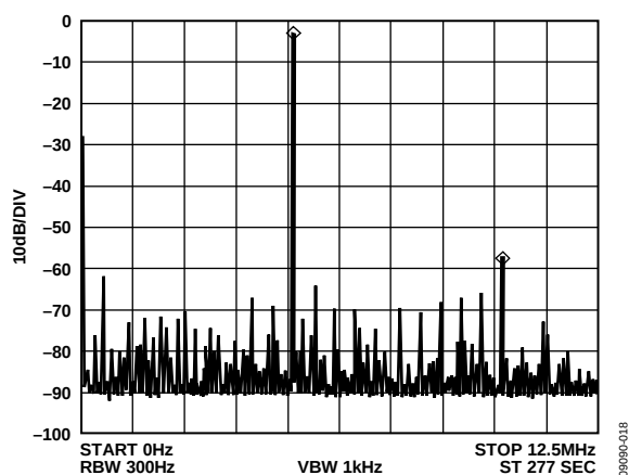
Figure 18. f_{MCLK} = 25 MHz, f_{OUT} = 5.1 MHz, Frequency Word = 0x34395810
