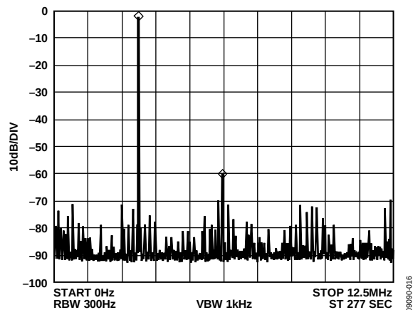
Figure 16. f_{MCLK} = 25 MHz, f_{OUT} = 3.1 MHz, Frequency Word = 0x1FBE76C9
