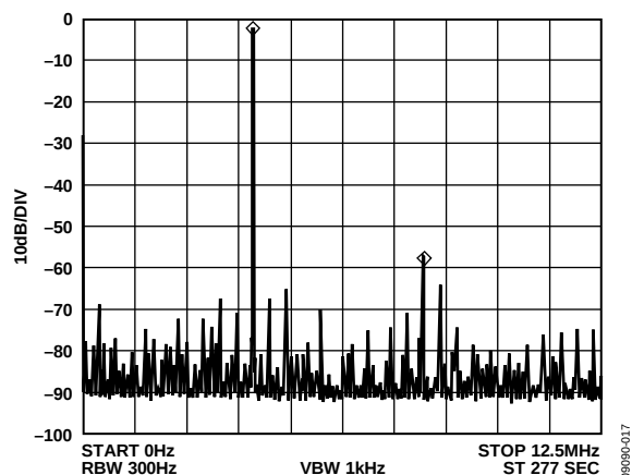
Figure 17. f_{MCLK} = 25 MHz, f_{OUT} = 4.1 MHz, Frequency Word = 0x29FBE76D
