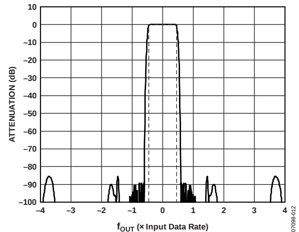
Figure 57. 8× Interpolation, Low-Pass Response to \pm 4\times Input Data Rate (Dotted Lines Indicate 1 dB Roll-Off)
