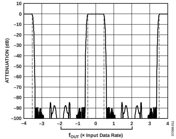
Figure 56. 4× Interpolation, Low-Pass Response to \pm 4\times Input Data Rate (Dotted Lines Indicate 1 dB Roll-Off)
