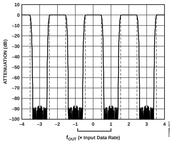
Figure 55. 2× Interpolation, Low-Pass Response to \pm 4\times Input Data Rate (Dotted Lines Indicate 1 dB Roll-Off)
