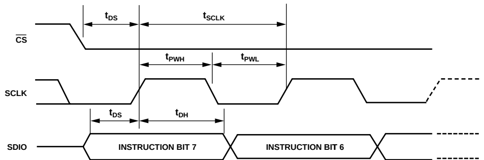
Figure 35. Timing Diagram for Register Write to AD9777
