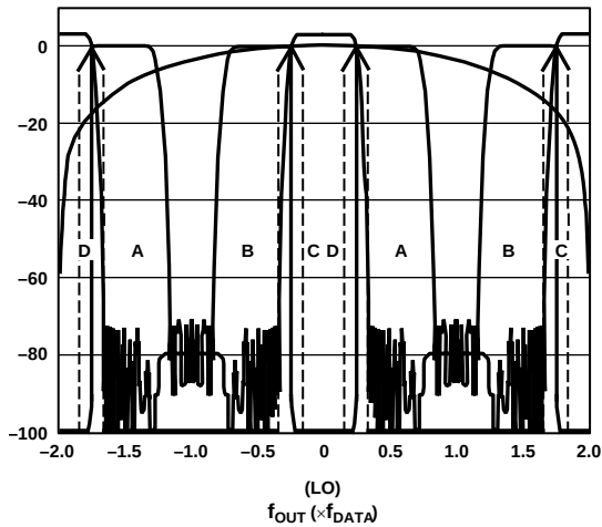
Figure 86. 2× Interpolation, Complex f_{DAC}/8 Modulation
