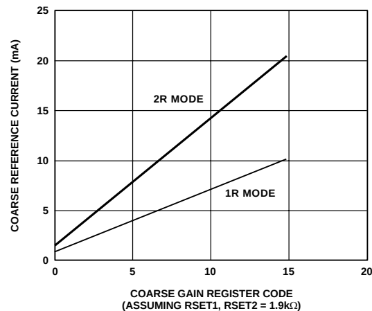
Figure 38. Coarse Gain Effect on I_{FULLSCALE}
