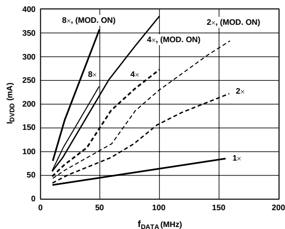
Figure 49. I_{\text{DVDD}} vs. f_{\text{DATA}} vs. Interpolation Rate, PLL Disabled
