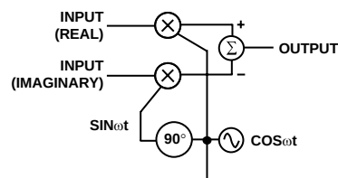
Figure 78. Quadrature Modulator
