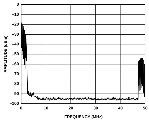
Figure 89. AD9775 Real DAC Output of Complex Input Signal Near Baseband (Positive Frequencies Only), Interpolation = 4×, No Modulation in AD9775
