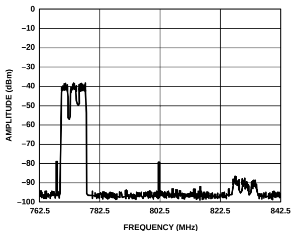
Figure 100. AD9775/AD8345 Synthesizing a Three-Carrier W-CDMA Signal at an LO of 800 MHz
