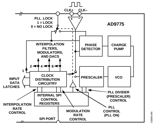
Figure 46. PLL and Clock Circuitry with PLL Disabled
