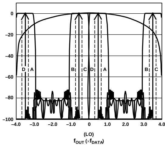
Figure 87. 4× Interpolation, Complex f_{DAC}/8 Modulation
