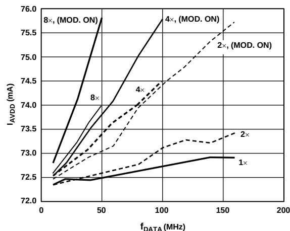
Figure 50. I_{\text{AVDD}} vs. f_{\text{DATA}} vs. Interpolation Rate, PLL Disabled
