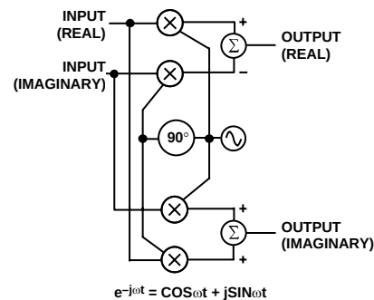
Figure 77. Implementation of a Complex Modulator
