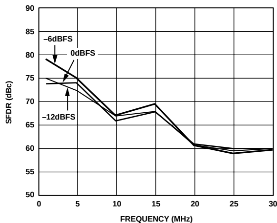
Figure 11. Out-of-Band SFDR vs. f_{\text{OUT}} @ f_{\text{DATA}} = 78\text{ MSPS}
