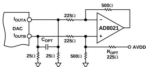
Figure 99. Op Amp-Coupled Output Circuit
