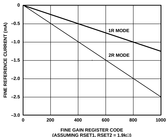
Figure 39. Fine Gain Effect on I_{FULLSCALE}
