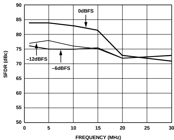
Figure 10. In-Band SFDR vs. f_{\text{OUT}} @ f_{\text{DATA}} = 78\text{ MSPS}
