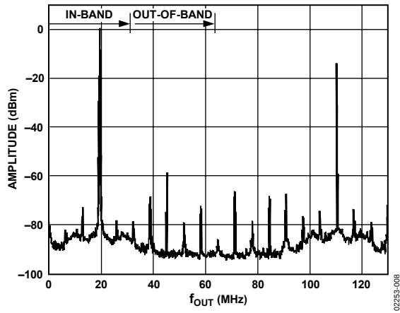
Figure 8. Single-Tone Spectral Characteristics @ f_{\text{DATA}} = 65 MSPS with f_{\text{OUT}} = f_{\text{DATA}}/3
