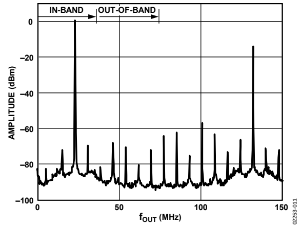
Figure 11. Single-Tone Spectral Characteristics @ f_{\text{DATA}} = 78 MSPS with f_{\text{OUT}} = f_{\text{DATA}}/3
