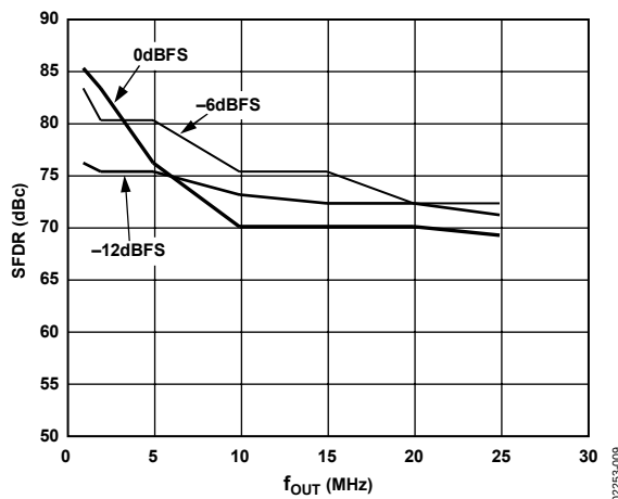
Figure 9. In-Band SFDR vs. f_{\text{OUT}} @ f_{\text{DATA}} = 65 MSPS
