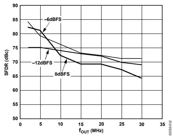
Figure 12. In-Band SFDR vs. f_{\text{OUT}} @ f_{\text{DATA}} = 78 MSPS
