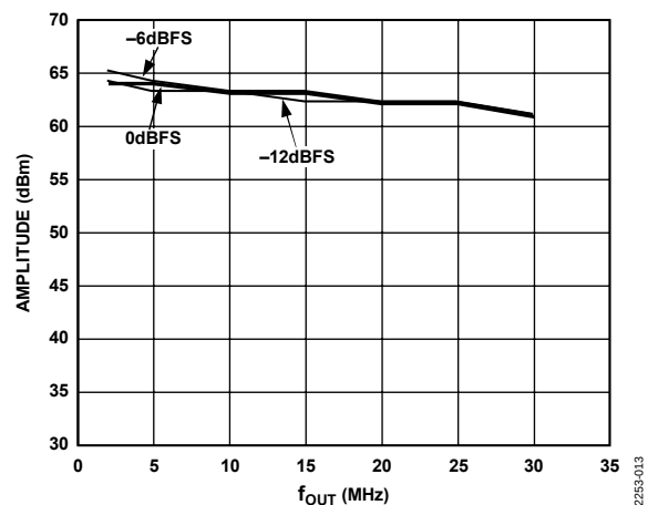
Figure 13. Out-of-Band SFDR vs. f_{\text{OUT}} @ f_{\text{DATA}} = 78 MSPS
