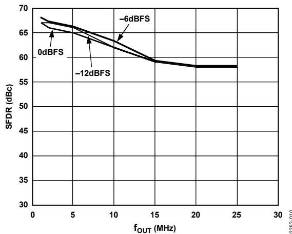
Figure 10. Out-of-Band SFDR vs. f_{\text{OUT}} @ f_{\text{DATA}} = 65 MSPS
