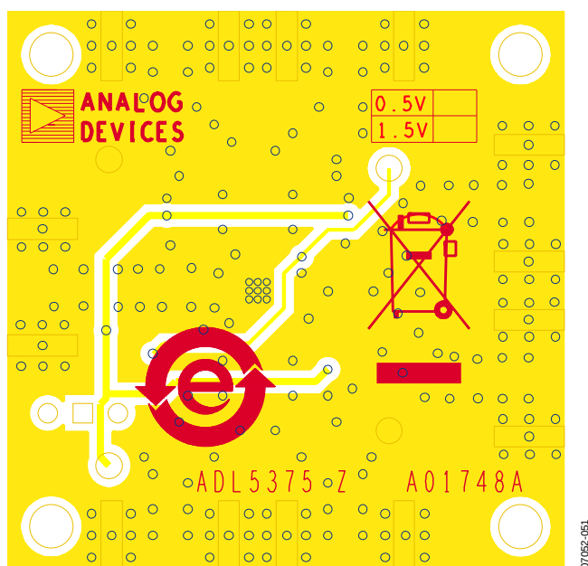
Figure 72. Evaluation Board Layout, Bottom Layer
