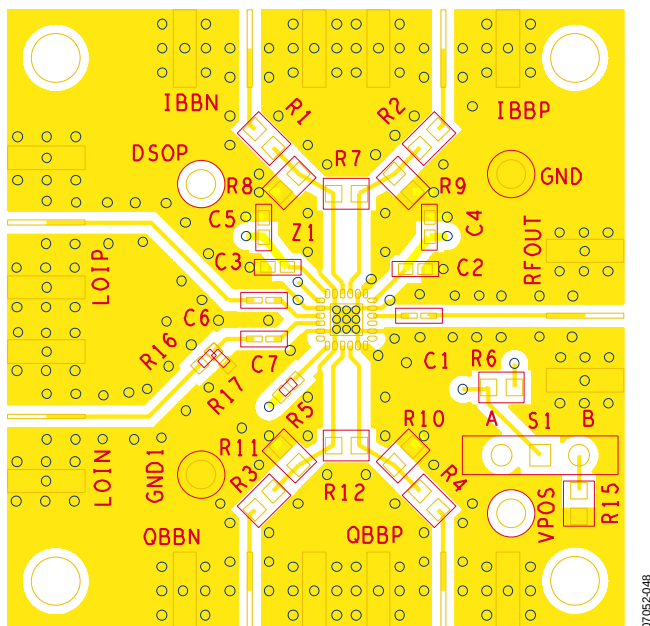
Figure 71. Evaluation Board Layout, Top Layer
