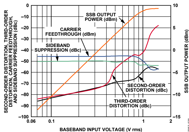
Figure 38. Second- and Third-Order Distortion, Carrier Feedthrough, Sideband Suppression, and SSB P_{OUT} vs. Baseband Differential Input Level ( f_{LO} = 900 MHz)
