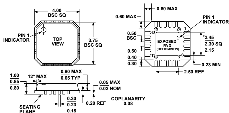
Figure 40. 24-Lead Lead Frame Chip Scale Package [LFCSP_VQ] 4 mm x 4 mm Body, Very Thin Quad (CP-24-2)
