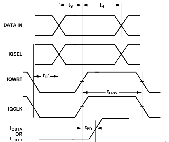
Figure 65. 5 V Only Interleaved Mode Timing
