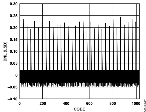
Figure 17. Typical DNL
