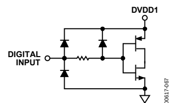
Figure 67. Equivalent Digital Input
