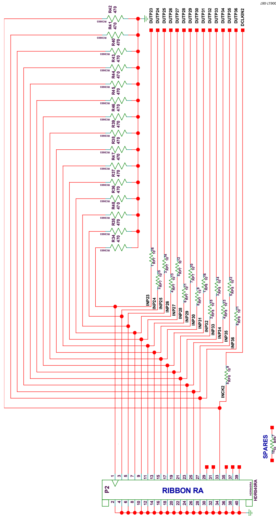
Figure 90. Digital Input Signaling (2)
