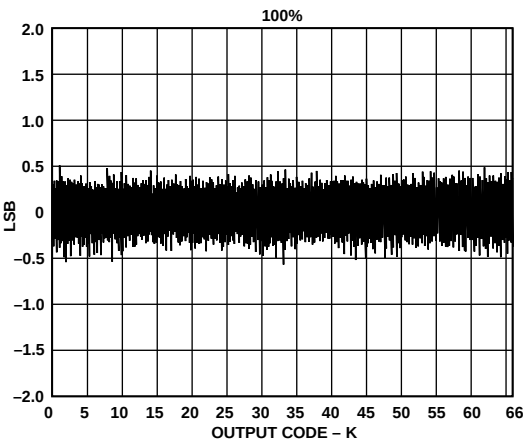
Figure 12. DNL Plot
