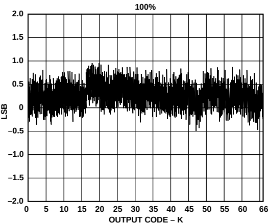
Figure 11. INL Plot
