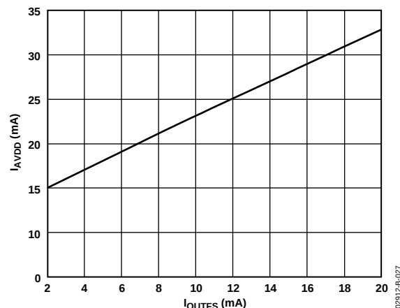
Figure 28. I_{AVDD} vs. I_{OUTFS}
