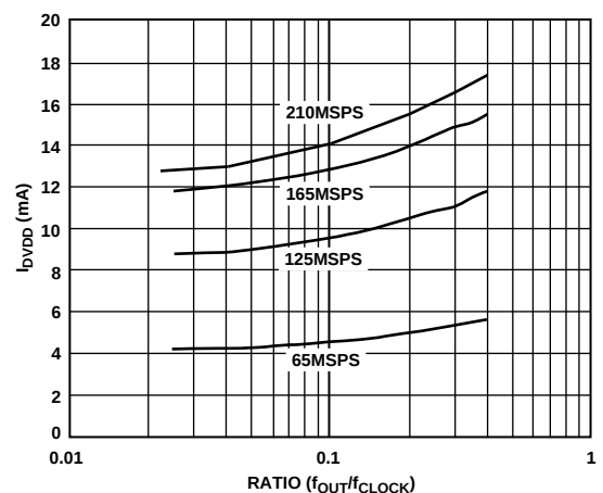
Figure 29. I_{DVDD} vs. Ratio @ DVDD = 3.3 V
