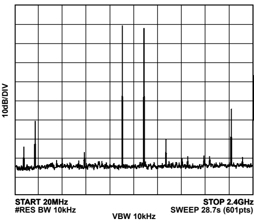
Figure 28. Single-Tone Spectrum in Mix Mode at f_{OUT} = 1.31 GHz, f_{DAC} = 2.4 GSPS
