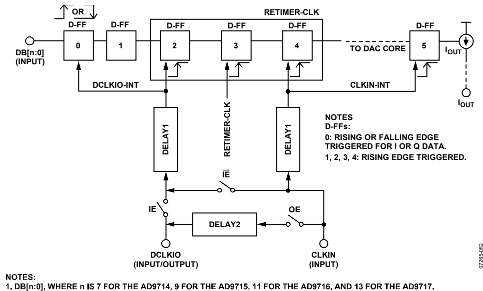
Figure 94. Simplified Diagram of AD9714/AD9715/AD9716/AD9717 Timing
