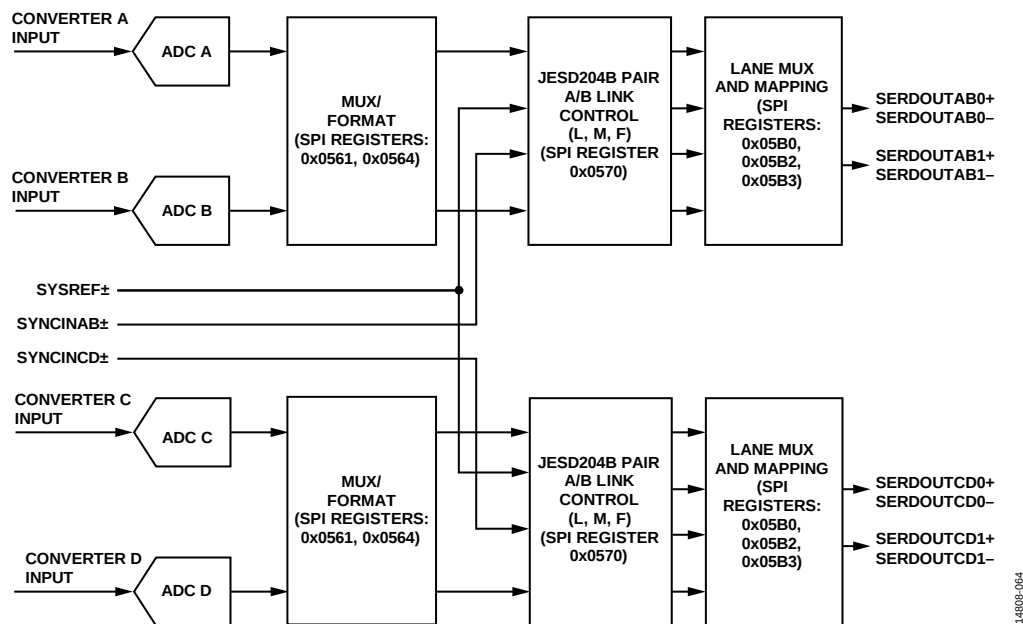
Figure 81. Transmit Link Simplified Block Diagram Showing Full Bandwidth Mode (Register 0x0200 = 0x00)
