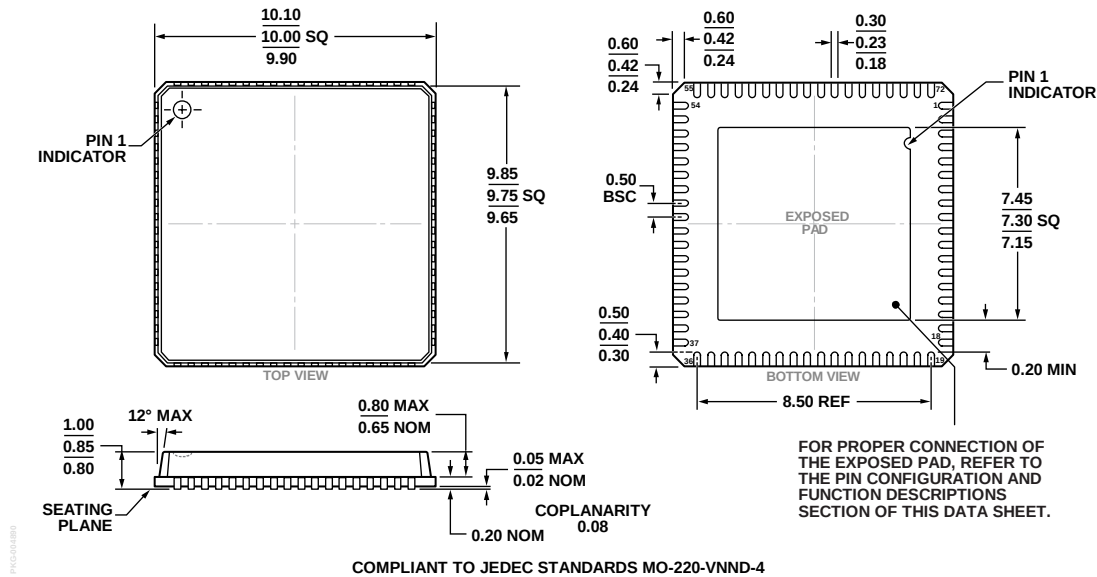
Figure 108. 72-Lead Lead Frame Chip Scale Package [LFCSP] 10 mm × 10 mm Body and 0.85 mm Package Height (CP-72-10)
