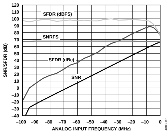
Figure 21. SNR/SFDR vs. Analog Input Frequency, f_{IN} = 155 MHz
