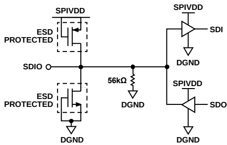
Figure 51. SDIO Input
