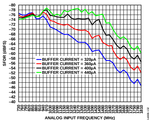
Figure 35. SFDR vs. Analog Input Frequency with Different Buffer Current Settings (Fourth Nyquist Zone)
