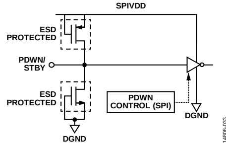
Figure 53. PDWN/STBY Input
