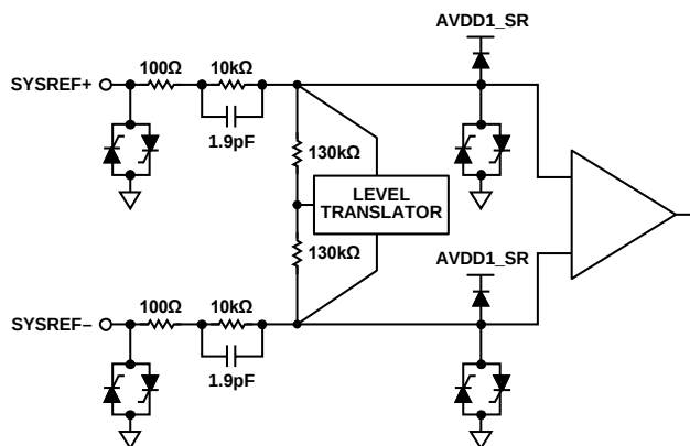
Figure 46. SYSREF± Inputs
