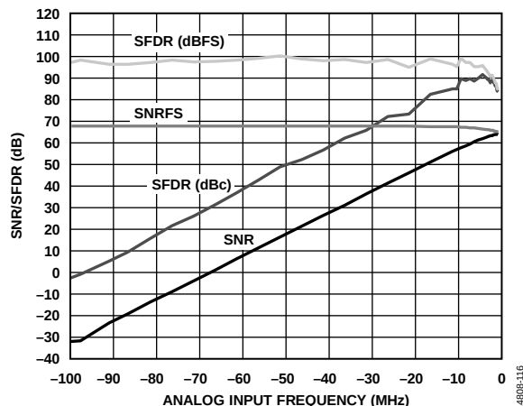
Figure 22. SNR/SFDR vs. Analog Input Frequency, f_{IN} = 305 MHz
