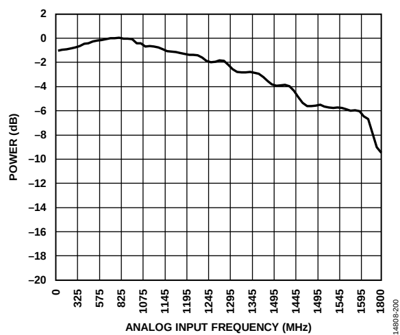
Figure 43. Full Power Bandwidth
