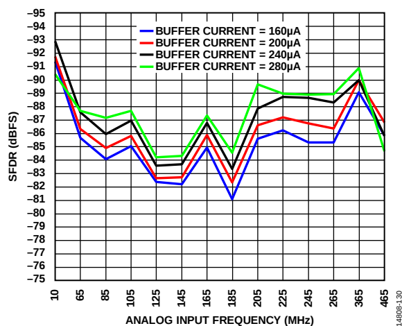
Figure 33. SFDR vs. Analog Input Frequency with Different Buffer Current Settings (First and Second Nyquist Zones)
