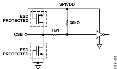
Figure 59. CSB Input
