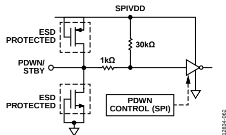
Figure 62. PDWN/STBY Input
