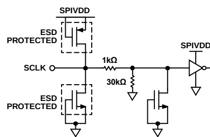
Figure 58. SCLK Input
