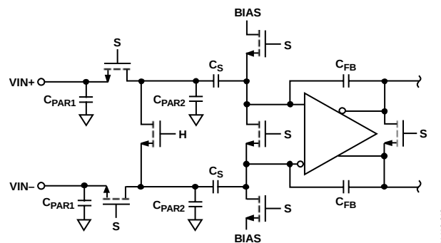
Figure 43. Switched Capacitor Input
