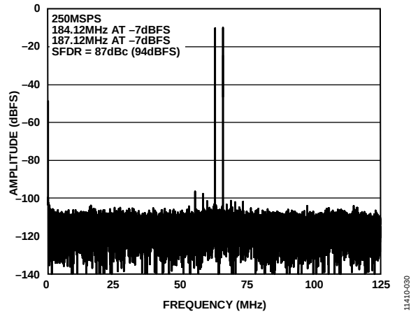
Figure 30. AD9683-250 Two-Tone FFT with f_{IN1} = 184.12 MHz, f_{IN2} = 187.12 MHz, f_S = 250 MSPS
