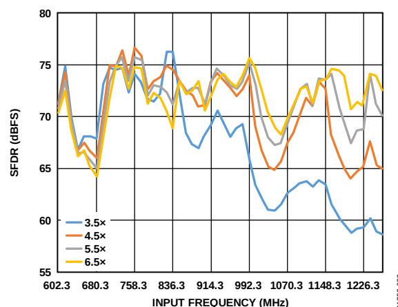
Figure 119. Buffer Current Sweeps, AD9680-1250 (SFDR vs. I_{BUFF} ); 600 \text{ MHz} < f_{IN} < 1300 \text{ MHz} ; Front-End Network Shown in Figure 115
