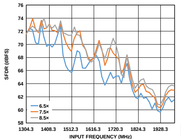
Figure 120. Buffer Current Sweeps, AD9680-1250 (SFDR vs. I_{BUFF} ); 1300 \text{ MHz} < f_{IN} < 2000 \text{ MHz} ; Front-End Network Shown in Figure 115
