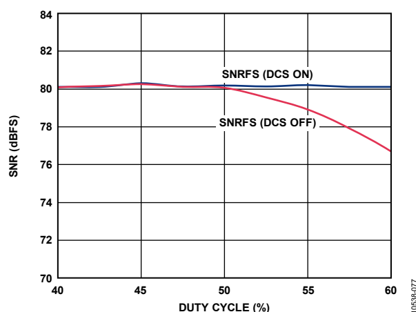
Figure 68. SNR vs. DCS On/Off, V_{REF} = 1.3\text{ V}
