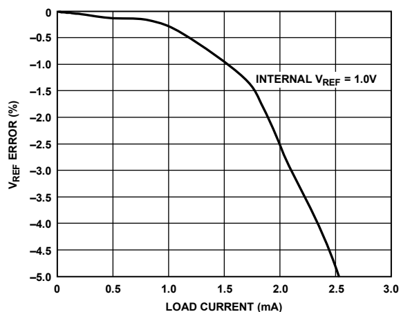
Figure 58. V_{REF} = 1.0\text{ V} Error vs. Load Current
