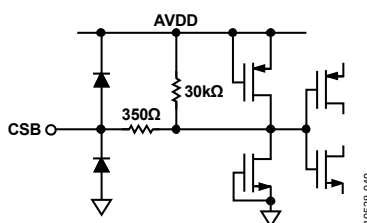
Figure 49. Equivalent \overline{CS} Input Circuit
