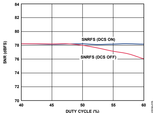
Figure 67. SNR vs. DCS On/Off, V_{REF} = 1.0\text{ V}
