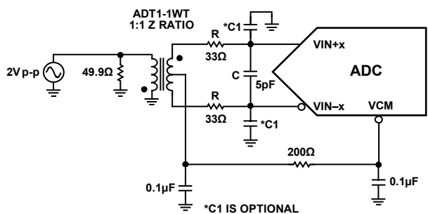
Figure 57. Differential Transformer-Coupled Configuration for Baseband Applications
