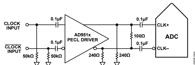
Figure 64. Differential PECL Sample Clock (Up to 1 GHz)
