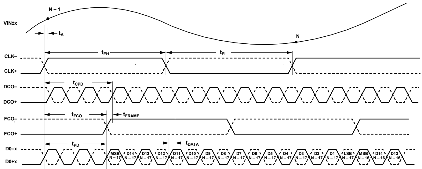
Figure 4. Wordwise DDR, One-Lane, 1x Frame, 16-Bit Output Mode
