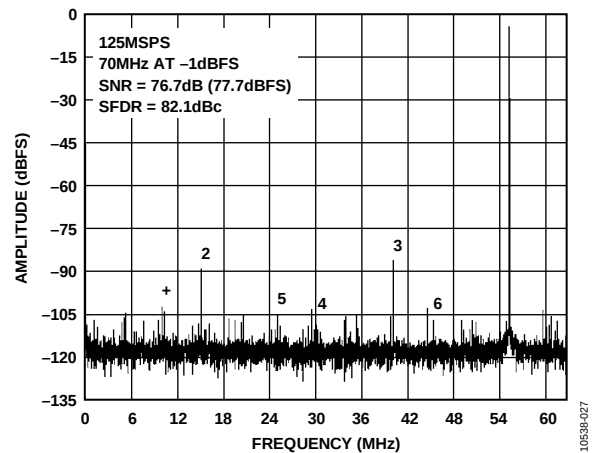
Figure 27. Single-Tone 16k FFT with f_{IN} = 70\text{ MHz} , f_{SAMPLE} = 125\text{ MSPS} , V_{REF} = 1.3\text{ V}
