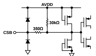
Figure 49. Equivalent \overline{CS} Input Circuit
