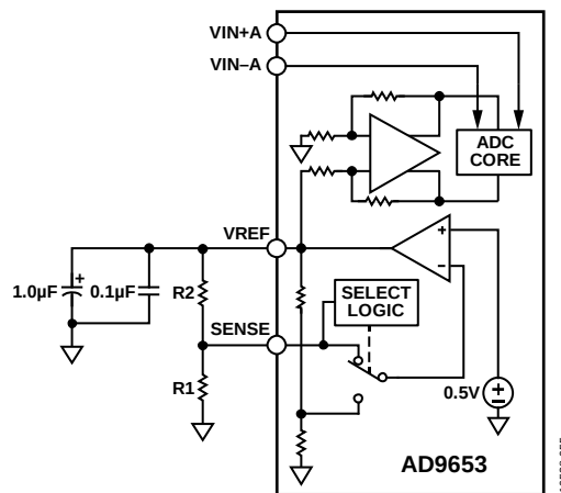
Figure 55. Programmable Internal Reference Configuration
