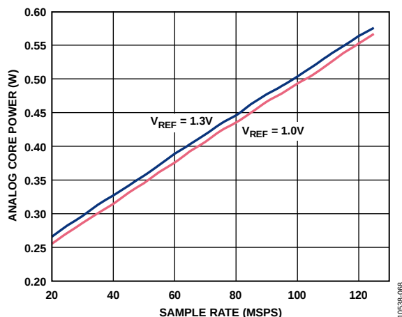
Figure 70. Analog Core Power vs. f_{\text{SAMPLE}} for f_{\text{IN}} = 9.7 MHz, Four Channels
