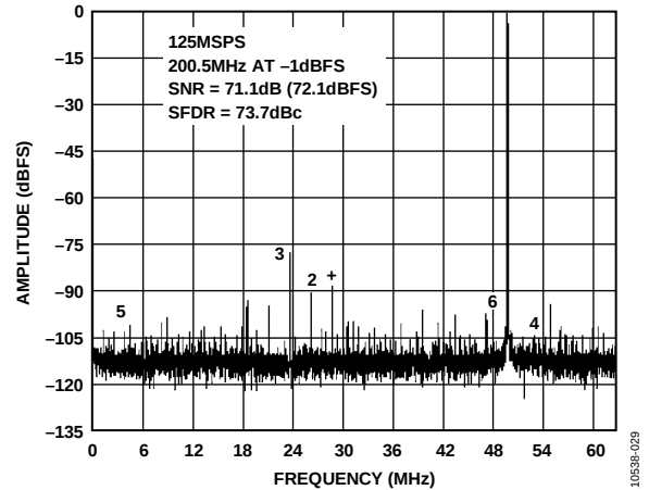
Figure 29. Single-Tone 16k FFT with f_{IN} = 200.5\text{ MHz} , f_{SAMPLE} = 125\text{ MSPS} , V_{REF} = 1.3\text{ V}
