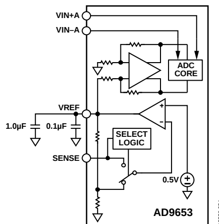
Figure 54. 1.0 V Internal Reference Configuration
