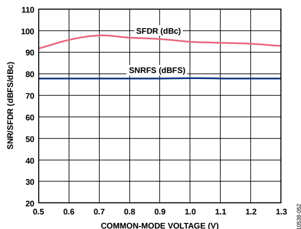
Figure 52. SNR/SFDR vs. Common-Mode Voltage, f_{IN} = 9.7 \text{ MHz} , f_{SAMPLE} = 125 \text{ MSPS} , V_{REF} = 1.0 \text{ V}
