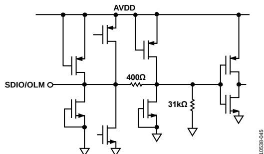
Figure 45. Equivalent SDIO/OLM Input Circuit
