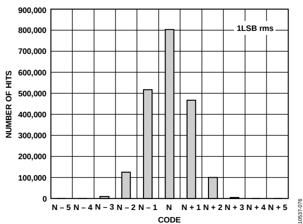
Figure 39. Input Referred Noise Histogram; f_{SAMPLE} = 125 MSPS
