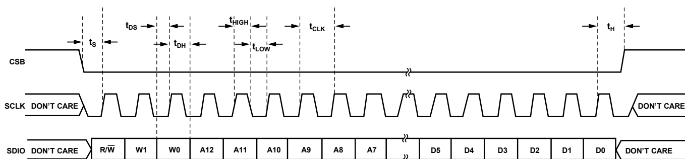
Figure 68. Serial Port Interface Timing Diagram
