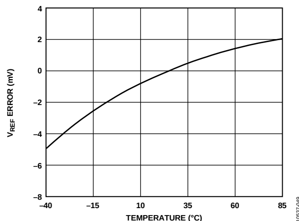
Figure 54. Typical V_{\text{REF}} Drift
