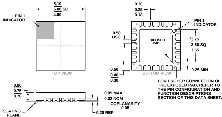
Figure 70. 32-Lead Lead Frame Chip Scale Package [LFCSP_WQ] 5 mm × 5 mm Body, Very Very Thin Quad (CP-32-12) Dimensions shown in millimeters
