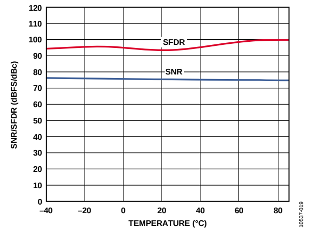
Figure 19. SNR/SFDR vs. Temperature; f_{IN} = 9.7 MHz, f_{SAMPLE} = 80 MSPS
