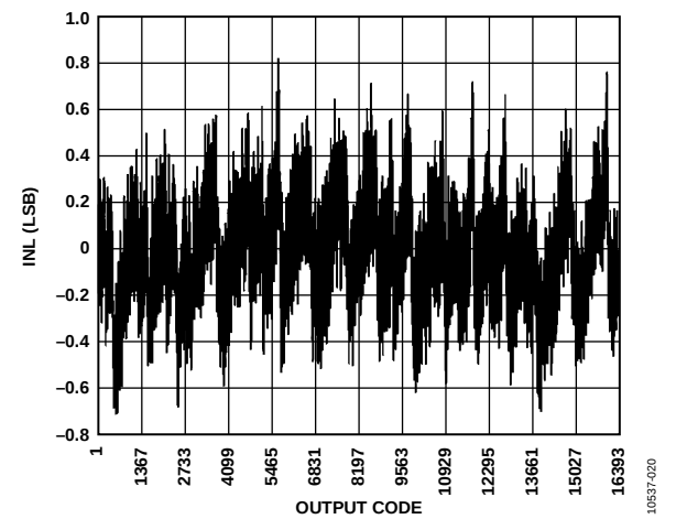
Figure 20. INL; f_{IN} = 9.7 MHz, f_{SAMPLE} = 80 MSPS
