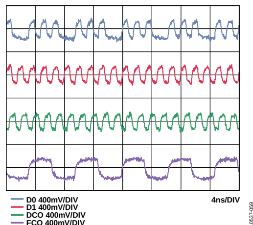
Figure 65. AD9645-125, LVDS Output Timing Example in Reduced Range Mode
