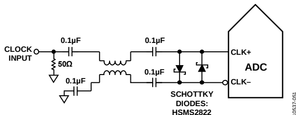
Figure 58. Balun-Coupled Differential Clock (Up to 1 GHz)
