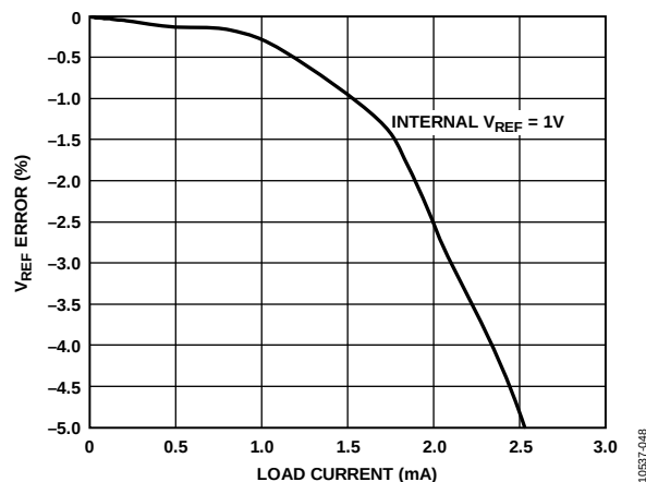
Figure 53. V_{\text{REF}} Error vs. Load Current
