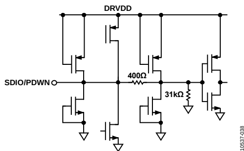
Figure 45. Equivalent SDIO/PDWN Input Circuit
