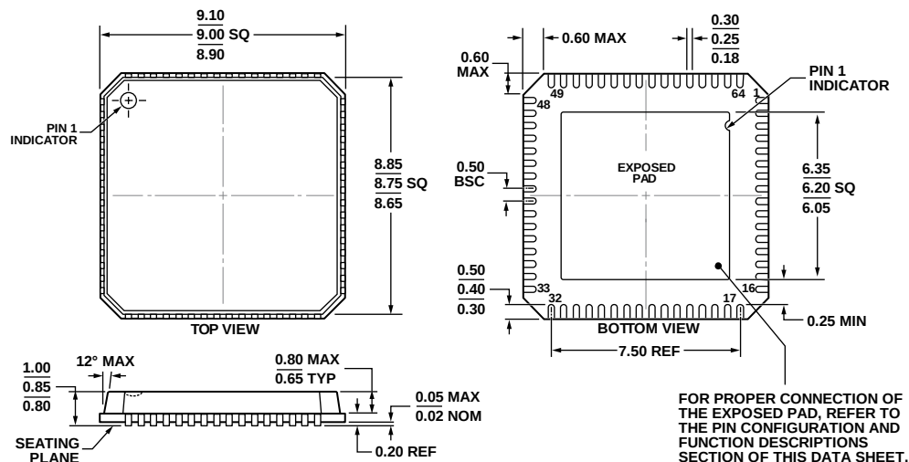
Figure 59. 64-Lead Lead Frame Chip Scale Package [LFCSP_VQ] 9 mm × 9 mm Body, Very Thin Quad (CP-64-4)
