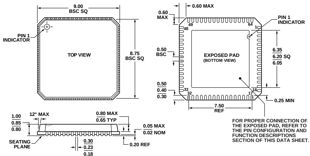
Figure 59. 64-Lead Lead Frame Chip Scale Package [LFCSP_VQ]
