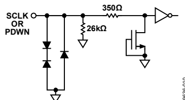
Figure 43. Equivalent SCLK or PDWN Input Circuit
