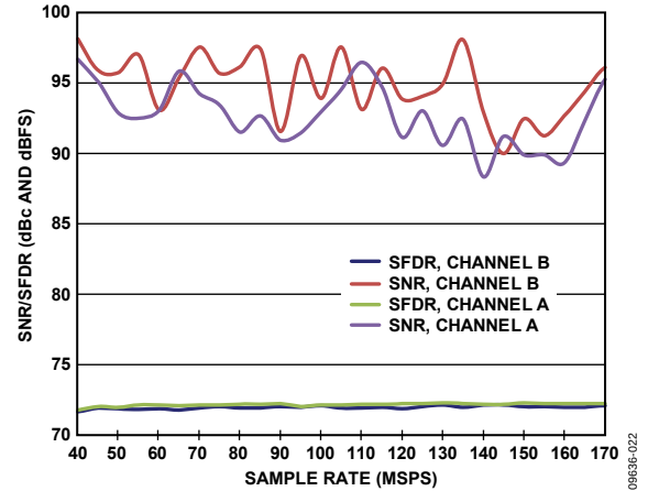
Figure 15. AD9643-170 Single-Tone SNR/SFDR vs. Sample Rate ( f_s ) with f_{IN} = 90.1 MHz
