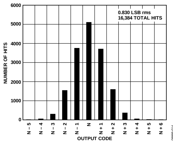
Figure 15. AD9642-170 Grounded Input Histogram, f_s = 170 MSPS
