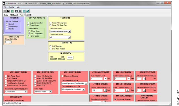
Figure 12. SPI Controller, Example ADC A Tab
