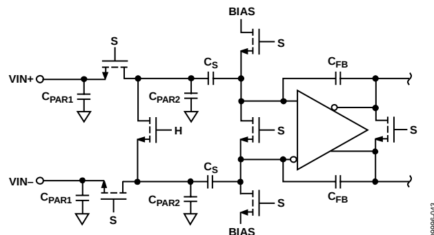
Figure 46. Switched-Capacitor Input
