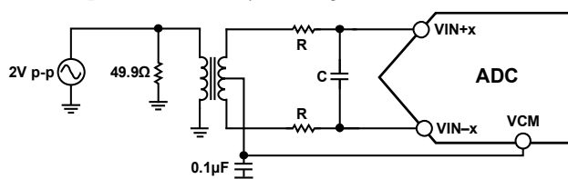
Figure 45. Differential Transformer-Coupled Configuration
