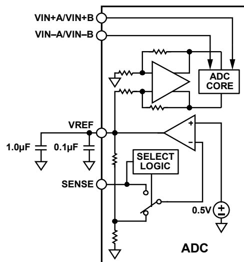
Figure 48. Internal Reference Configuration
