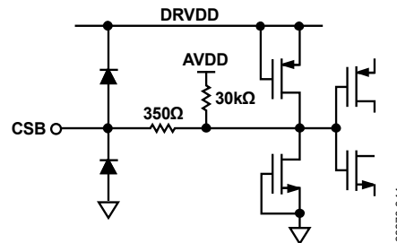
Figure 40. Equivalent CSB Input Circuit
