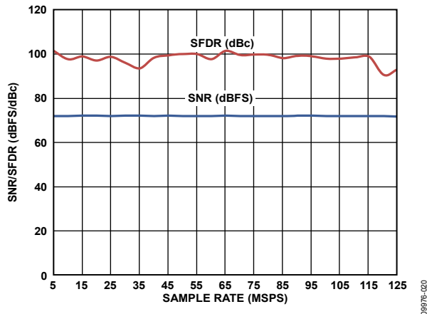
Figure 16. SNR/SFDR vs. Sample Rate with AIN = 9.7 MHz
