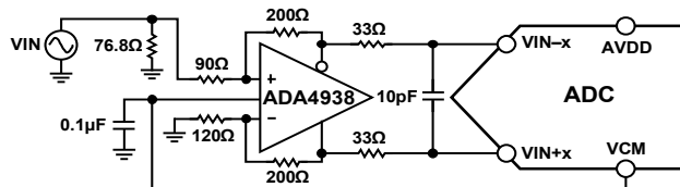
Figure 44. Differential Input Configuration Using the ADA4938-2
