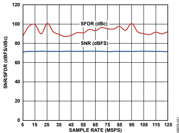
Figure 19. SNR/SFDR vs. Sample Rate with AIN = 70 MHz
