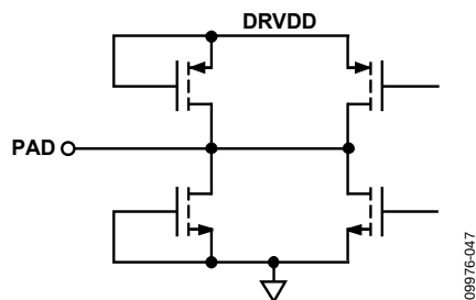
Figure 36. Equivalent Digital Output Circuit
