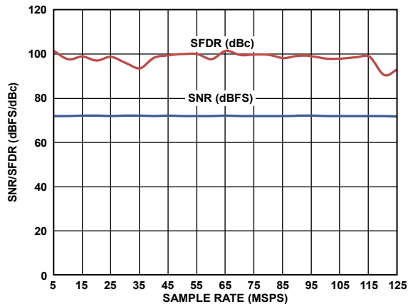
Figure 16. SNR/SFDR vs. Sample Rate with A_{IN} = 9.7 MHz
