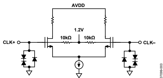
Figure 5. Clock Inputs
