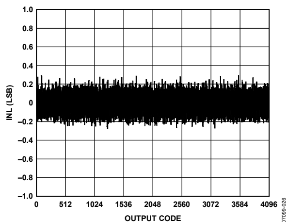
Figure 17. AD9626-170 INL; 170 MSPS
