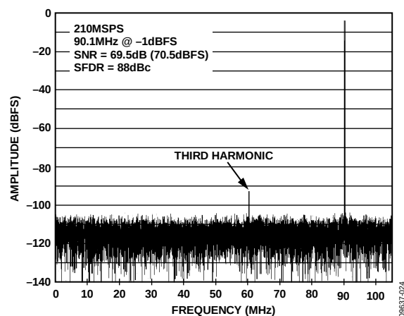
Figure 17. AD9613-210 Single-Tone FFT with f_{IN} = 90.1 MHz
