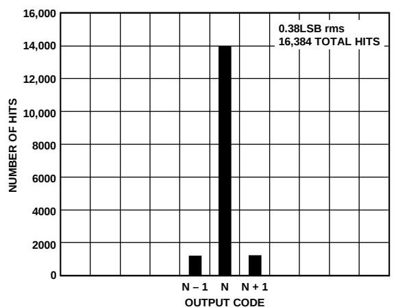
Figure 16. AD9613-170 Grounded Input Histogram
