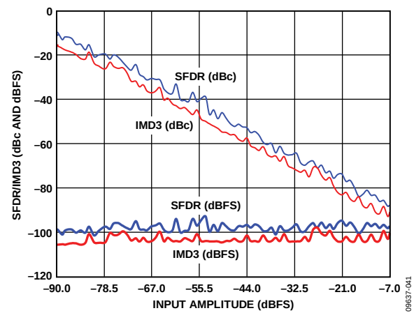
Figure 34. AD9613-250 Two-Tone SFDR/IMD3 vs. Input Amplitude ( A_{IN} ) with f_{IN1} = 184.12 , f_{IN2} = 187.12 MHz, f_s = 250 MSPS
