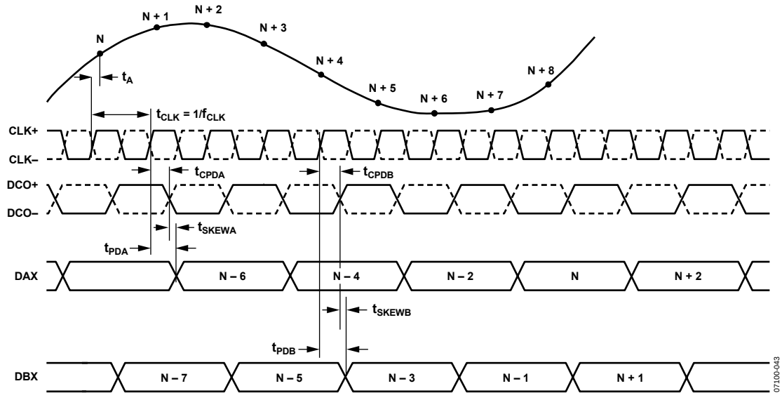
Figure 3. Interleaved Mode
