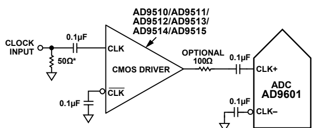
Figure 40. Single-Ended 3.3 V CMOS Sample Clock
