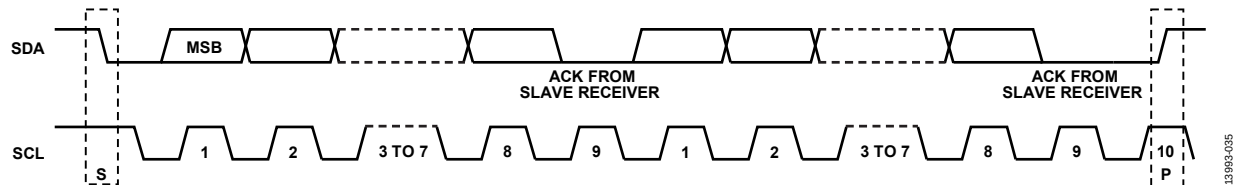
Figure 35. Acknowledge Bit
