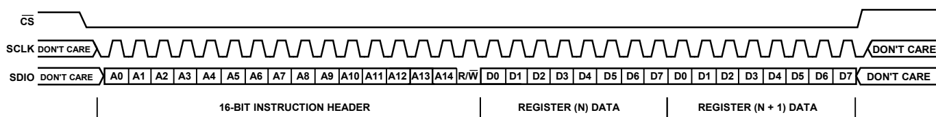
Figure 31. Serial Control Port Write—LSB First, Address Increment, Two Bytes of Data
