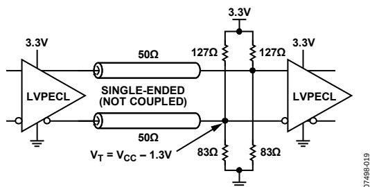
Figure 18. LVPECL Far-End Termination
