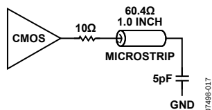
Figure 16. Series Termination of CMOS Output
