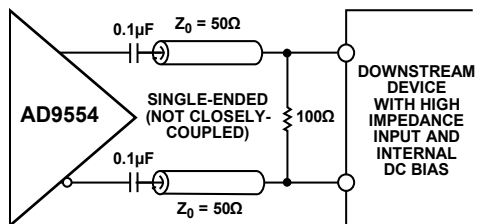
Figure 21. Destination Self-Biased Differential Receiver; Use 14 mA Mode for LVDS-Compatible Amplitude or 28 mA for LVPECL-Compatible Amplitudes (100 \Omega resistor must be as close to the destination receiver as possible.)
