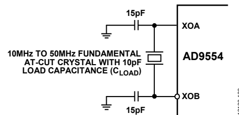
Figure 24. System Clock Input (XOA/XOB) in Crystal Mode (The recommended C_{LOAD} = 10 pF is shown. The values of 15 pF shunt capacitors shown here must equal 2 \times (C_{LOAD} - C_{STRAY}) , where C_{STRAY} is typically 2 pF to 5 pF.)
