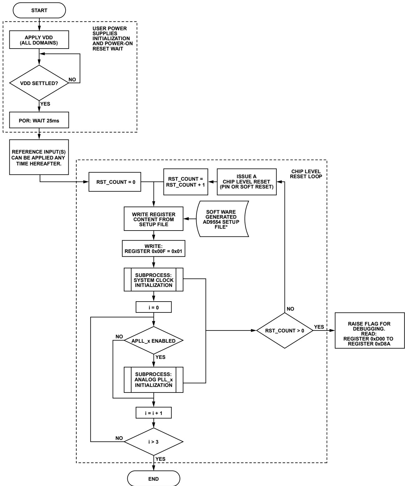
Figure 26. Main Process—Initialization
