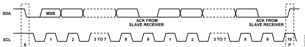
Figure 45. Acknowledge Bit
