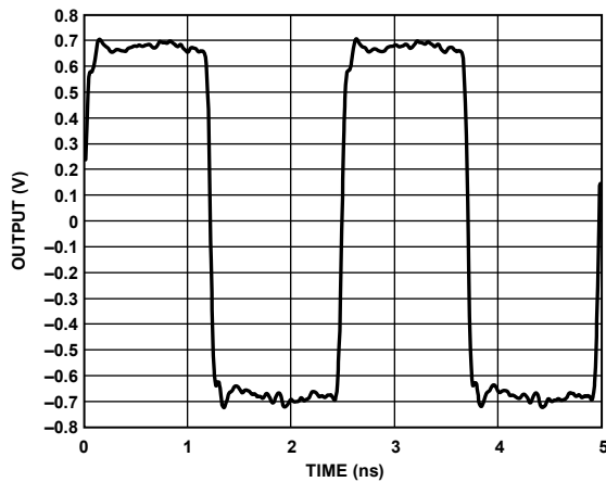
Figure 15. Output Waveform, 21 mA Mode (400 MHz) with 100 \Omega Termination at Load
