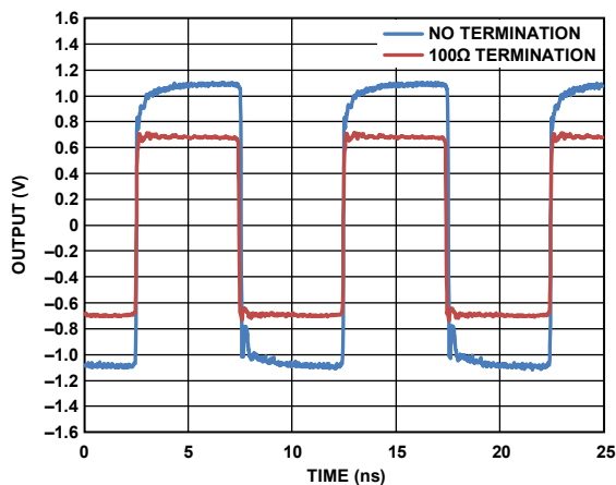
Figure 17. Output Waveform, 21 mA Mode (100 MHz)
