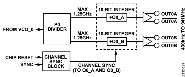
Figure 35. Clock Distribution Block Diagram from VCO_0 for the PLL_0
