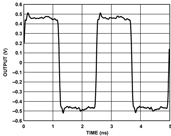
Figure 16. Output Waveform, 14 mA LVDS-Compatible Mode (400 MHz) with 100 \Omega Termination at Load
