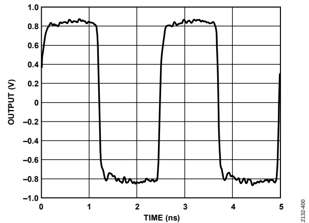
Figure 14. Output Waveform, 28 mA LVPECL-Compatible Mode (400 MHz) with 100 \Omega Termination Resistor
