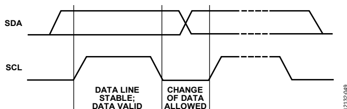
Figure 43. Valid Bit Transfer
